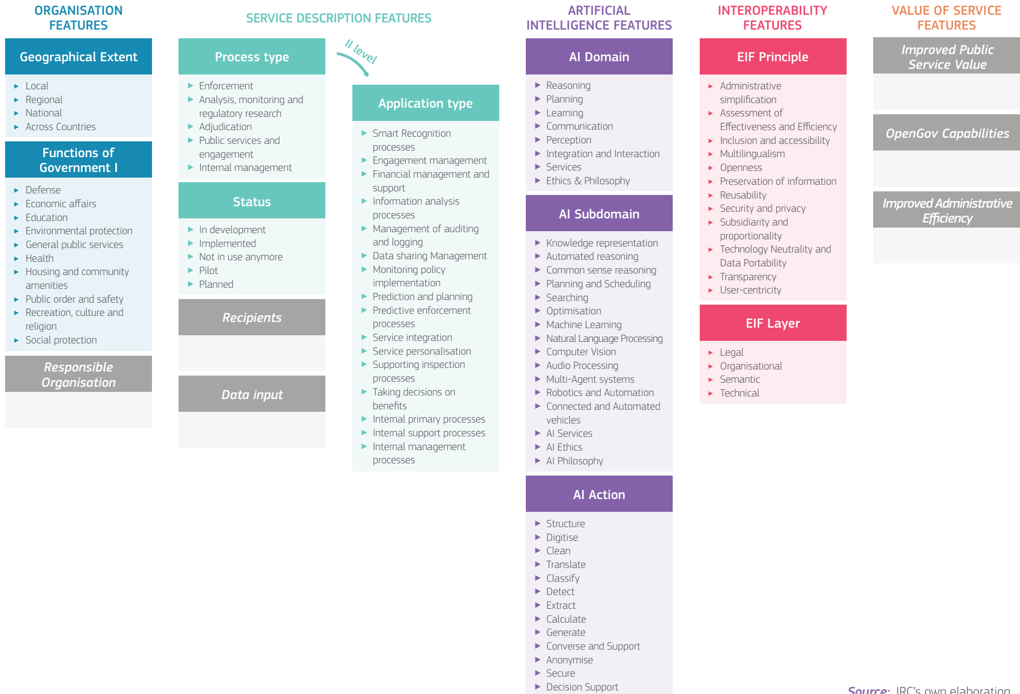
Figure 4. Taxonomy for AI case categorisation
